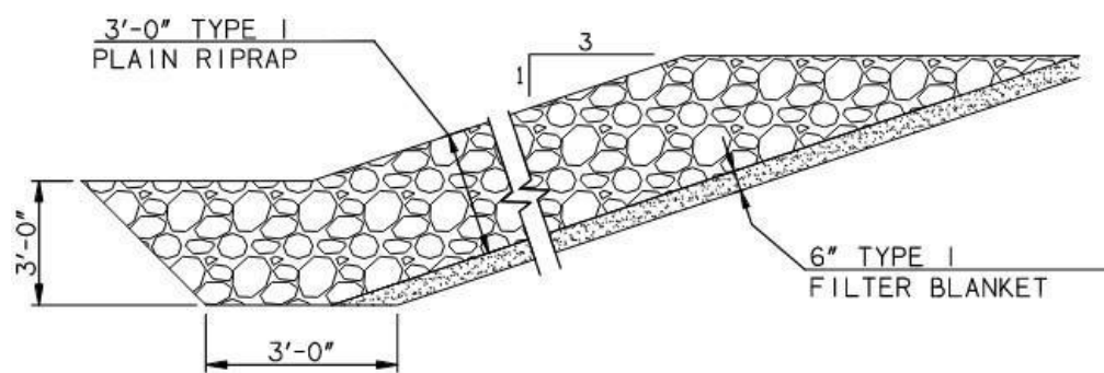
Typical riprap cross section
